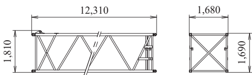
12.2 m Boom Insert (with Lug) Weight: 1,220 kg
