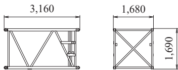
3.0 m Boom Insert Weight: 380 kg
