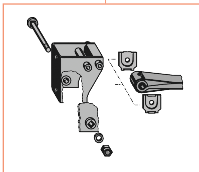
6 Spring Pivot Bolt Bearings
